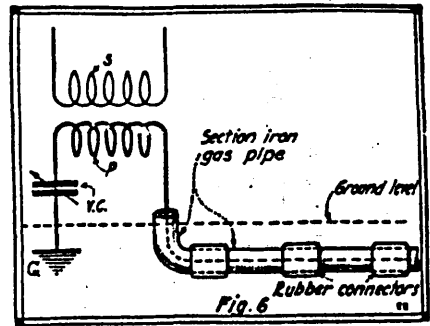
Here the Iron Pipe Jacket Surrounding the Buried Aerial is Divided up into 20-Foot Sections by Means of Rubber-Hose Connectors; a Later Development.
