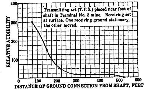
FIGURE 26.—Relation between audibility and distance between receiving grounds
