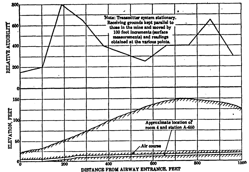
FIGURE 24.—Transmitting T. P. S. signals from inside experimental mine through overburden
